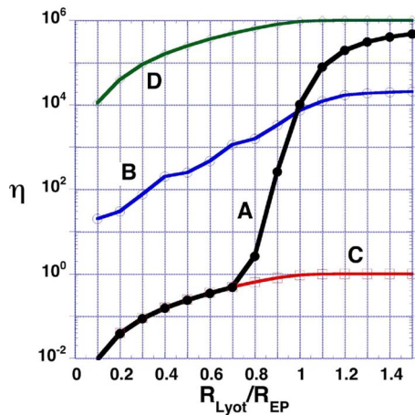
Fig. 5. A, Vortex and B, Lyot coronagraph performance curves for \alpha=2.2\lambda/R_{EP} where \eta represents the relative transmitted power. C, Ideal performance. D, Total relative transmitted power without filtering.
