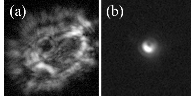
Fig. 3. (a). Image of a star (Betelgeuse) through a vortex lens without adaptive optics [28]. (b) Image of a star (Arcturus) through a vortex lens using adaptive optics.
