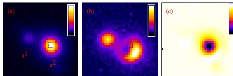
Fig. 5. Raw dark-frame-subtracted images of Cor Caroli in false color (a) without vortex, (b) with vortex, (c) difference with (a) subtracted from (b). The 2 \times 2 pixel outline in each image marks the registration position that produces the greatest difference.
