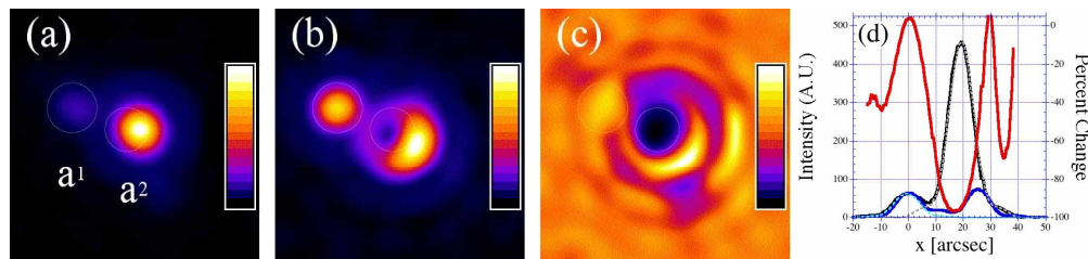
Fig. 6. Interpolated images (a) without vortex ( f_a ), (b) with vortex lens ( f_b ), (c) Relative difference, (f_b - f_a)/f_a . (d) Black line: Intensity plot through the peaks of the primary and secondary star without the vortex lens. Blue line: Same points with the vortex lens. Red line: the percent change that reaches -97%. Dashed lines: computer generated defocused point spread functions.
