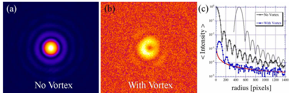
Fig. 4. False color laboratory measurements using a vortex coronagraph. (a) Without vortex lens. (b) With vortex lens. (c) Radially averaged intensity profiles of the data in (a) and (b). Black solid curve in (c) shifted to 4\lambda/D .
