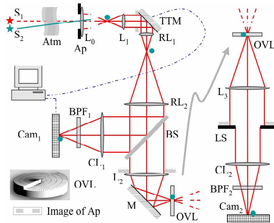
Fig. 1. Schematic diagram showing rays from a binary star system ( S_1 and S_2 ) passing through the atmosphere (Atm) and into a telescope comprised of an objective lens, L_0 , and subaperture, Ap. The rays are recollimated by lens L_1 whereby an image of Ap appears at the piezo-electrically driven tip-tilt mirror (TTM). A relay system, RL 1 and RL 2 , reproduces this image at the input face of lens L_2 . A 50/50 beam splitter (BS) directs light to a fast (500 Hz) camera, Cam 1 , whereby the star system is imaged by use of camera lens (CL 1 ). To correct the wavefront a computer sends a feedback signal to TTM. The remaining light is imaged on the optical vortex lens (OVL) by use of L_2 and recollimated by lens L_3 . A Lyot stop (LS) is positioned in the image plane of Ap, and the transmitted light forms a spatially filtered image of the star system on a telescope camera (Cam 2 ) by use of lens CL 2 . Both cameras employ bandpass filters (BPF). The surface of an OVL is illustrated in the inset.
