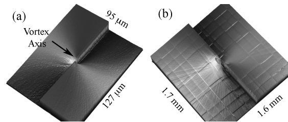
Fig. 2. Surface profile of the optical vortex lens in PMMA resist showing (a) relatively good surface quality in the central region containing the vortex axis, and (b) significant surface roughness owing to exposure non-uniformity near electron-beam field boundaries.
